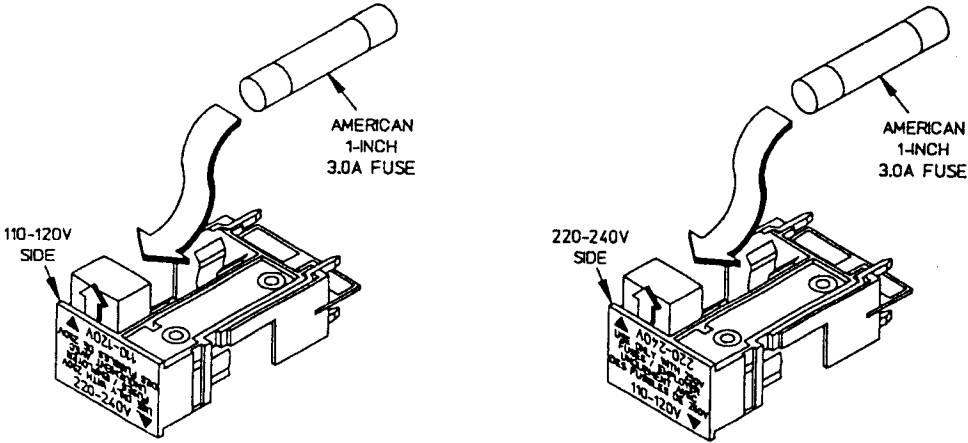
(b) CHECKING AND INSTALLING AMERICAN FUSE
