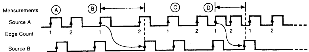
Source Sampling on Channel A (Edge Count = 2)
