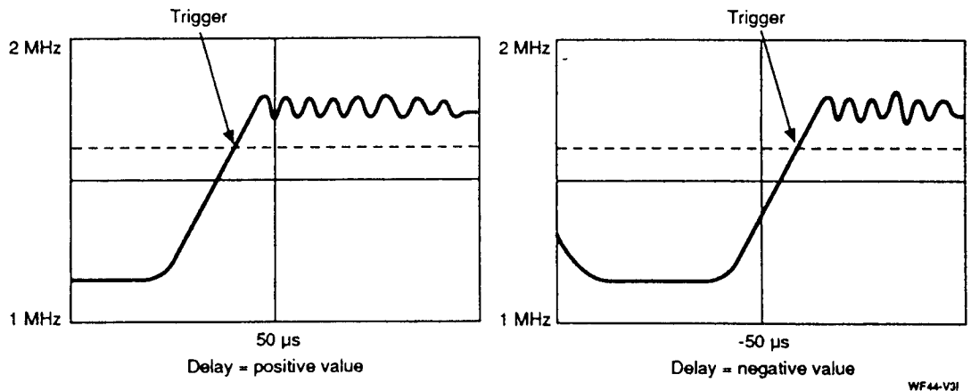
Figure 4-2. Illustration of the Delay Feature Using a Center Reference
