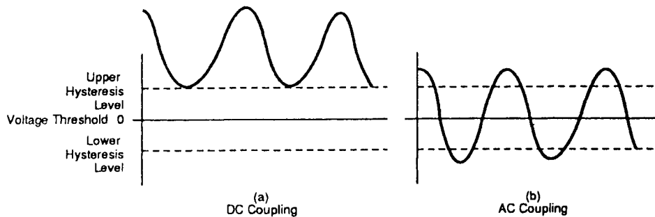
An input signal with the dc content shown in (a) would not be detected unless ac coupling was used (b) to remove the signal's dc content.
