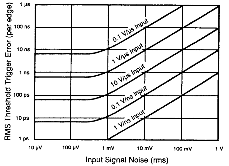
Graph 5 Noise on the input signal will add error to time interval measurements. Error is associated with both start and stop edges.
