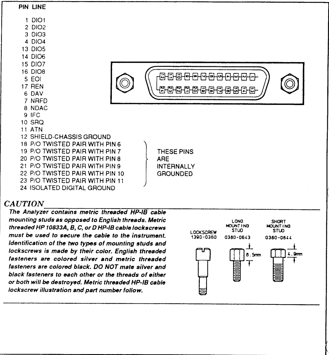
Figure A-5. Hewlett-Packard Interface Bus Connection
