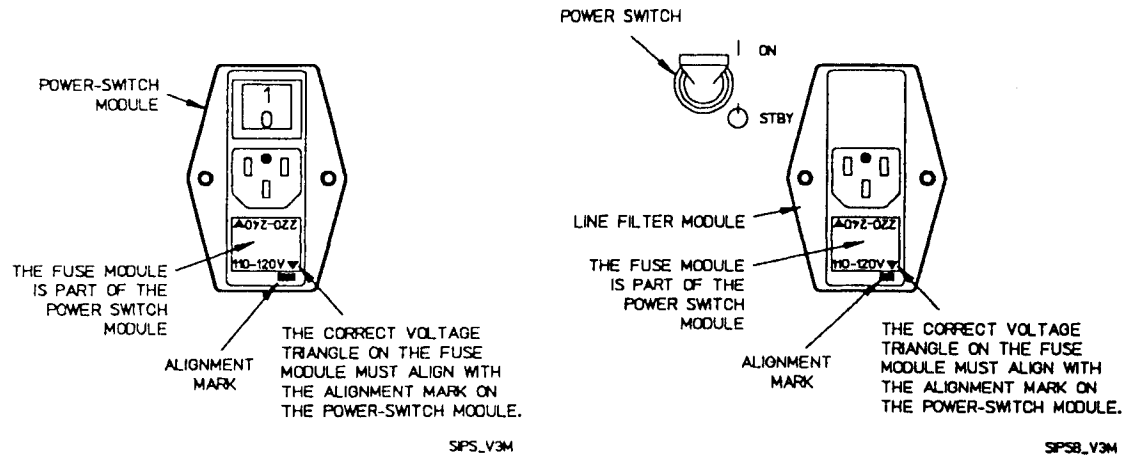
(a) Standard Instrument Power Module
