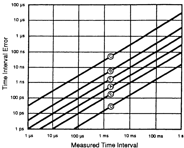
Graph 4 Time Interval Reference Error. Crystal aging will affect your Time Interval accuracy.
